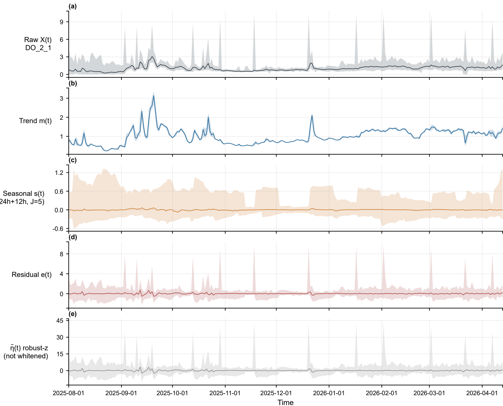
Full-span daily overview — DO_2_1 (aerobic, min) [2025-08-01~2026-04-13]
